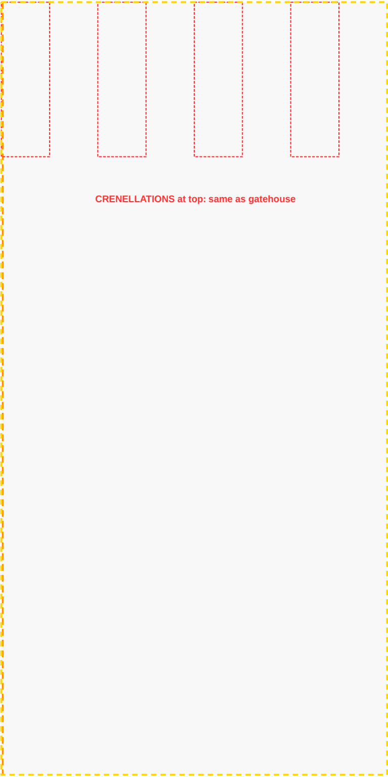
12" x 24" (30 x 61 cm) 2 panels per corner tower — tape at 90°
